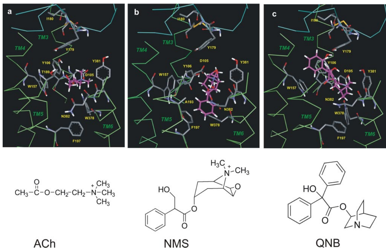
Fig. 5. Molecular model of the M_1 mAChR binding site docked with acetylcholine (a), S -(-)- N -methyl scopolamine (b), and R -(-)-3-quinuclidinyl benzilate (c).
