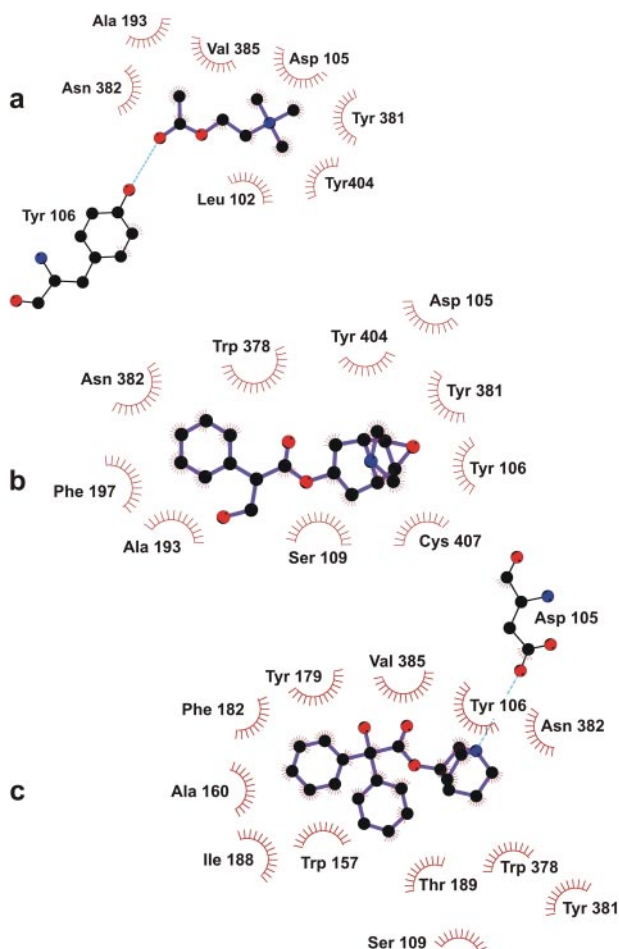
Fig. 6. 2-dimensional LIGPLOTS of the modeled M_1 mAChR binding site docked with acetylcholine (a), S -(-)- N -methyl scopolamine (b), and R -(-)-3-quinuclidinyl benzilate (c). Hatched semicircles indicate residues involved in hydrophobic contacts. Broken lines show hydrogen bonds; for ACh, the indicated H-bond length is 3.32 Å; for QNB, it is 2.86 Å.
